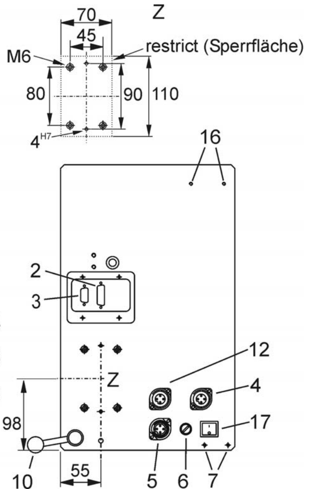
Fig. 2-5 Rear side of machine head microtap II
