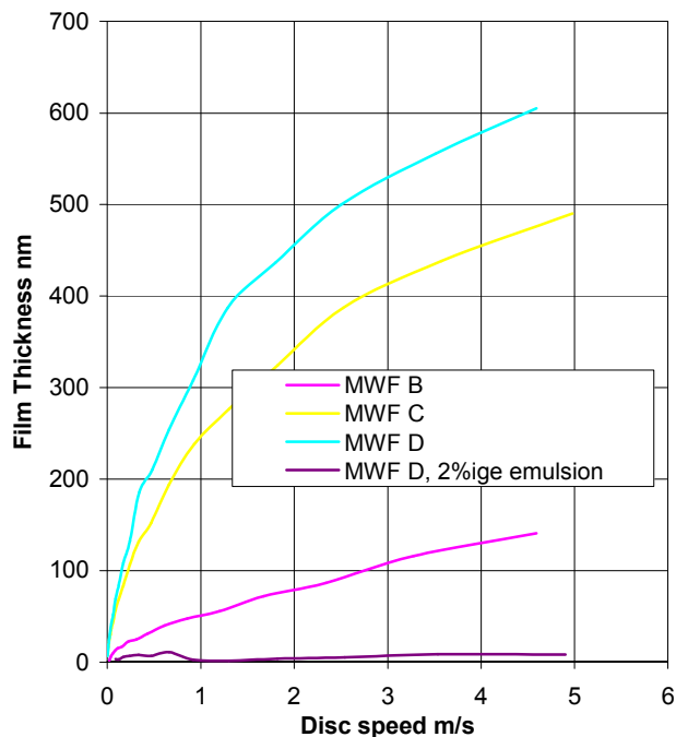
Figure 24: Optical Rig - Comparison film thickness concentrate/emulsion
