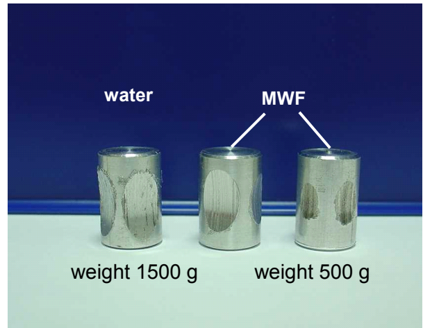
Figure 15: Wear scar on Al Mg Si0.5
