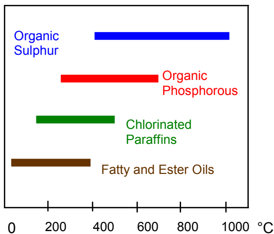
Figure 3: Activation temperature range of different lubrication additives
