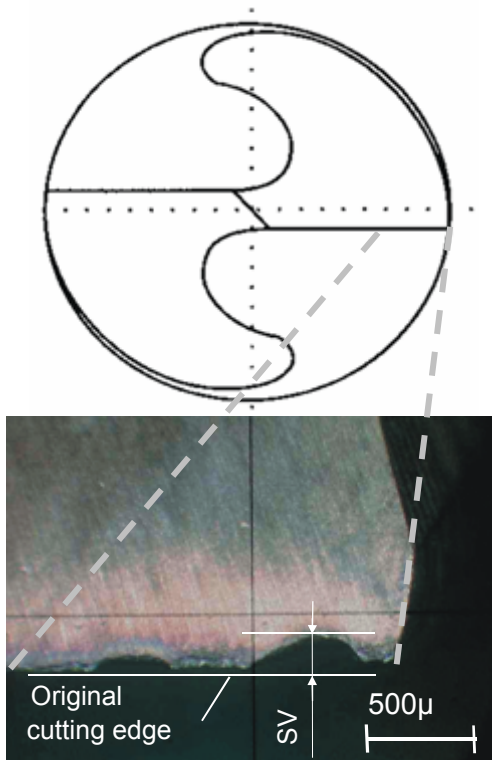
Figure 7: Cutting edge wear SV
