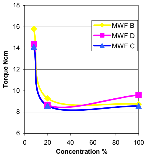
Figure 11: Thread cutting in Al Si18
