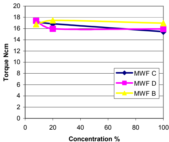
Figure 14: Thread cutting in GGG 60
