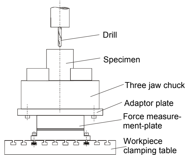
Figure 8: Experimental setup for drilling trial
