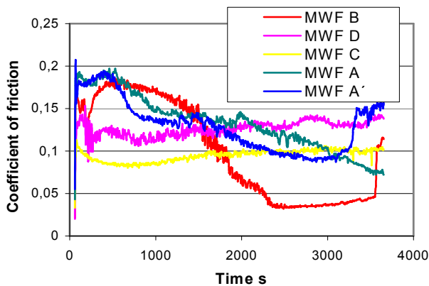
Figure 20: HFRR run with MWF concentrates
