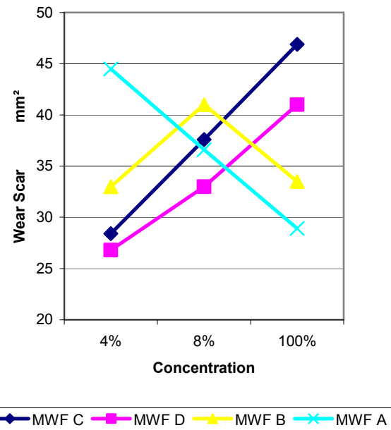
Figure 17: Reichert Al roll wear depending on MWF-concentration
