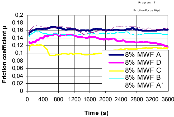
Figure 19: HFRR run with MWF emulsions, conc. 8 %
