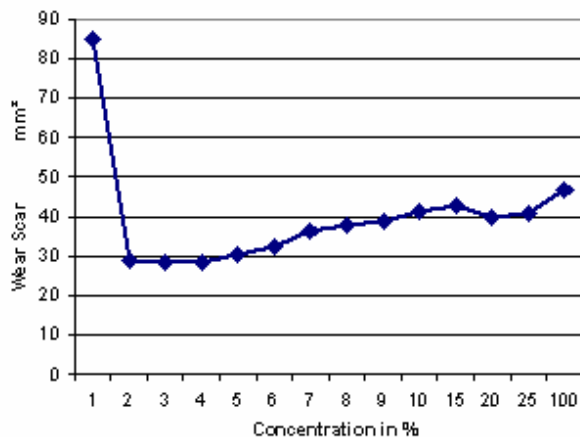
Figure 18: Reichert Al rolls activation concentration MWF C
