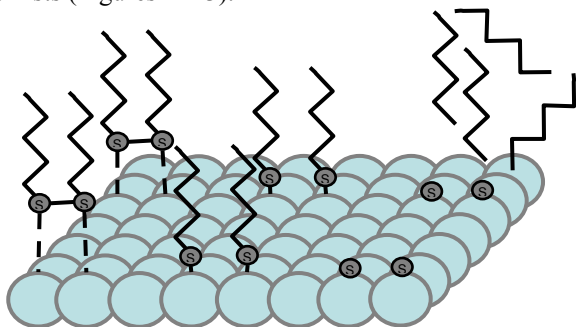
Physisorption Chemisorption Reaction Figure 2: Theoretical model of interaction between sulphur-carrier and metallic surface (S) [1]
