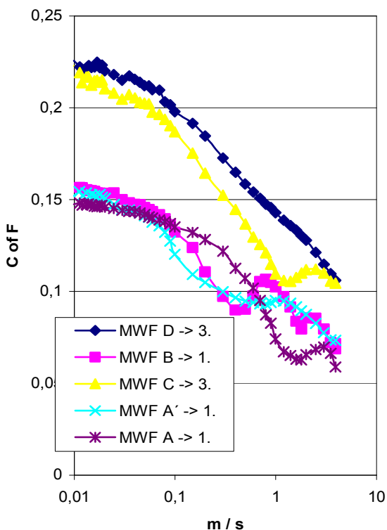
Figure 23: MTM Stribeck curves of 4 % concentration
