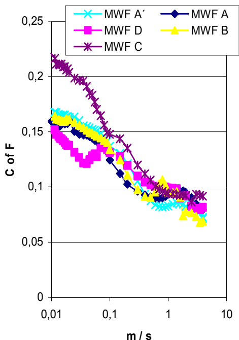
Figure 22: MTM Stribeck curves of MWF 8 % concentration
