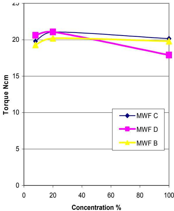
Figure 13: Thread cutting in 16 Mn Cr5
