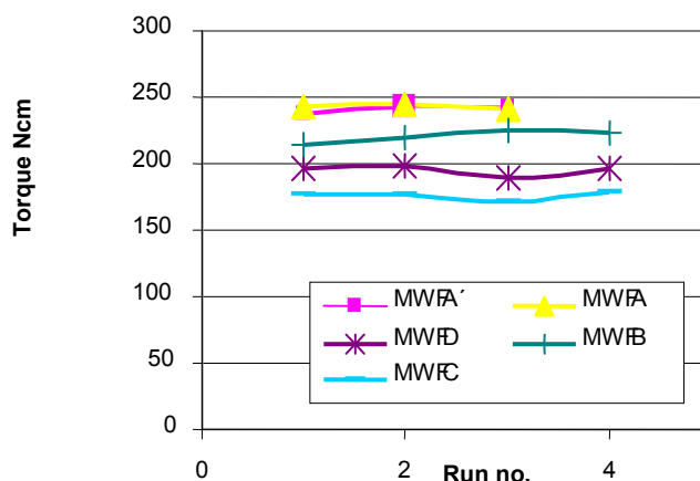
Figure 12: Thread Forming Al Mg Si0.5, MWF-conc. 8 %
