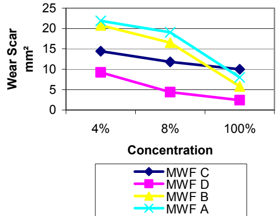
Figure 16: Reichert steel roll wear depending on MWF concentration
