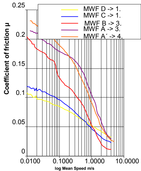
Figure 21: MTM Stribeck curves of MWF-concentrates
