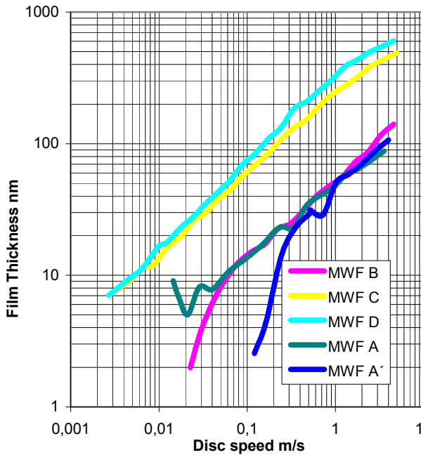
Figure 25: Optical Rig - Comparison of film thickness of different concentrates
