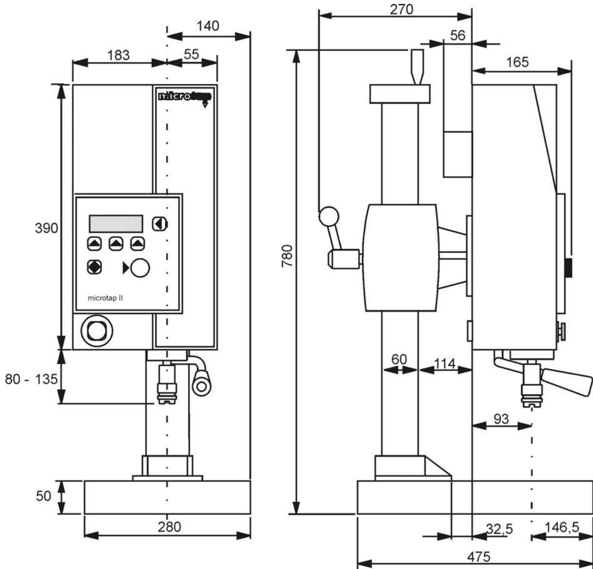
Dimensions microtap II (unit: mm)
